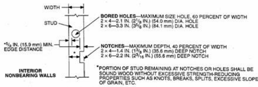
CUTTING, NOTCHING AND BORING OF STUDS
