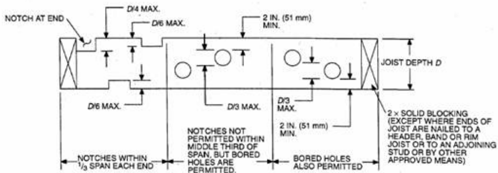
CUTTING, NOTCHING AND BORING OF FLOOR JOISTS
